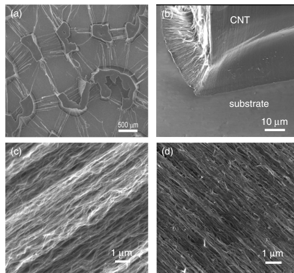
Figure 2. SEM images showing the structures formed by upright self-assembly of CNTs during the drying of a 1 mm CNT array synthesized on 1 nm Fe/Al 2 O 3 /Si catalyst. (a) Discrete islands; (b) an enlarged SEM image showing the bottom edge of a discrete island with no CNT lying down on the substrate surface; (c) and (d) showing the obvious change in the density of CNTs before and after the drying, respectively.
